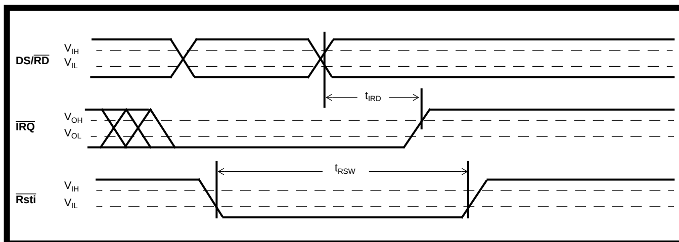
Figure 28 - INT &amp; Rsti Timing
